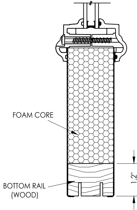
2 4 VERTICAL CROSS SECTION
