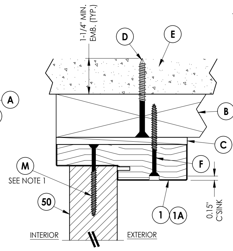
3 6 VERTICAL CROSS SECTION Inswing shown (Outswing similar) 2X Buck Construction
